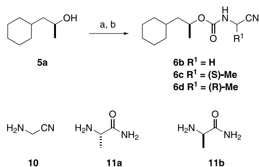
Scheme 3. Reagents and conditions: (a) 5a , 1.93 M COCl_2 in PhMe, pyridine, CH_2Cl_2 , -20\text{ }^\circ C to rt; 10 , 11a or b , i-Pr_2NEt , THF, 73–97%; (b) (CF_3CO)_2O , CH_2Cl_2 , 33–42%.
