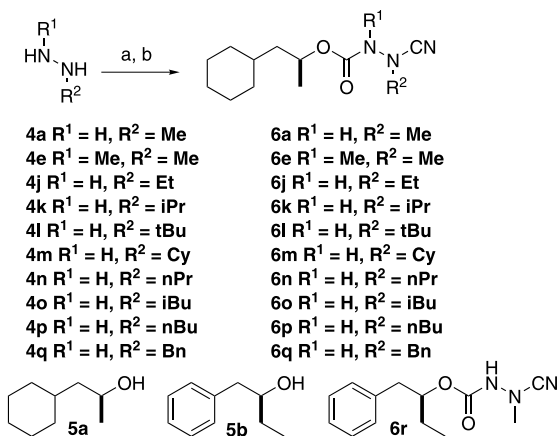
Scheme 1. Reagents and conditions: (a) BrCN, Na_2CO_3 , H_2O , CH_2Cl_2 , 67–96%; (b) 5a or b , 1.93 M COCl_2 in PhMe, pyridine, CH_2Cl_2 , -20\text{ }^\circ C to rt; cyanamide, i-Pr_2NEt , THF, 52–92%.
